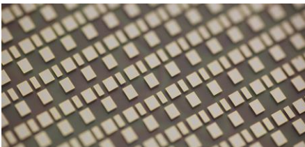
Donor Wafer with Cap Structures for Hermetic Transfer Bonding to Target Wafer
